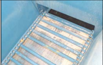
walking floor in hopper (hydraulically driven with flow control valve)
